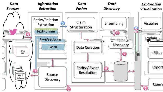
Figure 1: VERA Architecture
